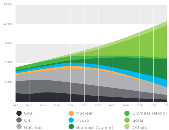
World primary Energy Consumption: Biomass & Solar Scenario 1990-2100
